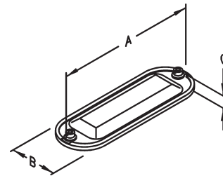
Raised Dome Stamped Aluminum Conduit Body Cover & Neoprene Gasket
